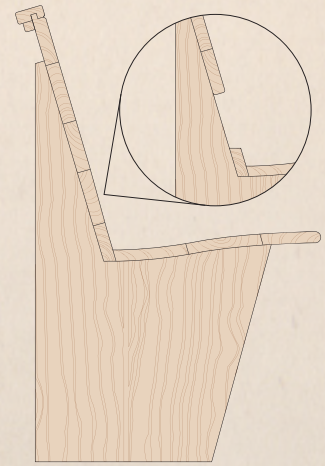
555 Pew End Available with a fully closed back or an opening across the bottom of the backrest
